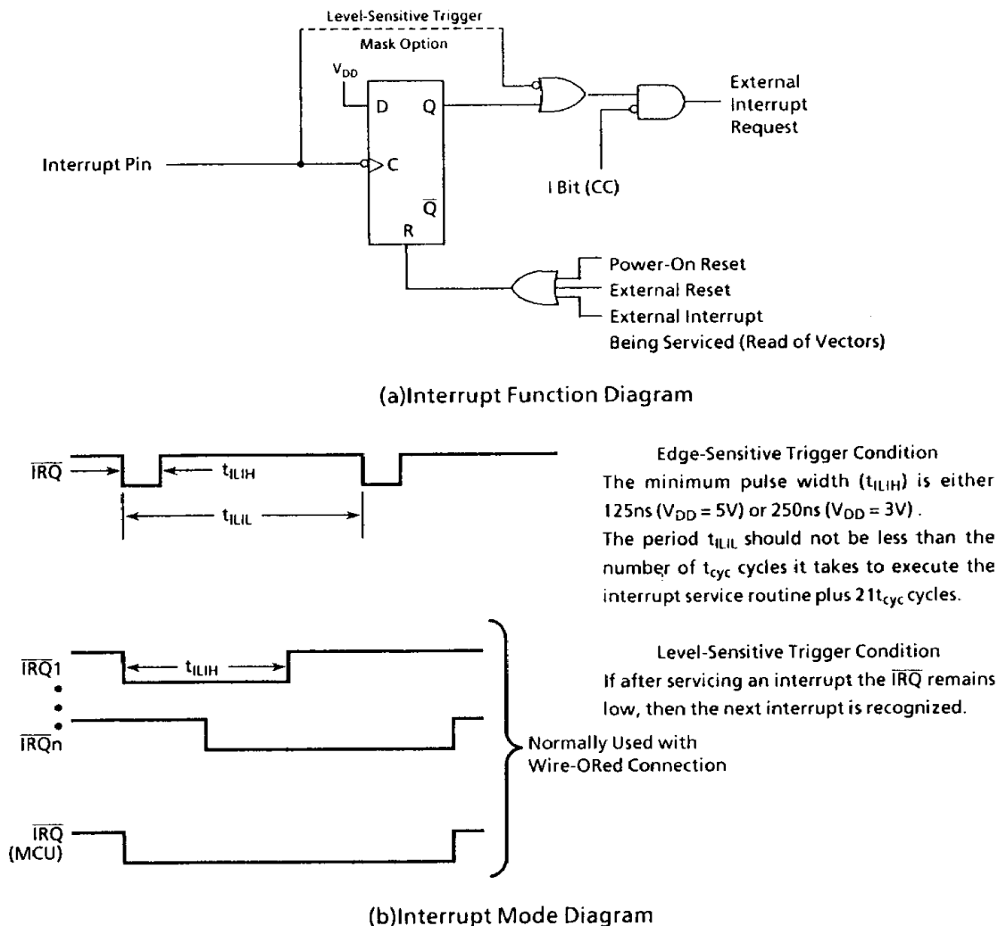
Figure 3.4 External Interrupt
