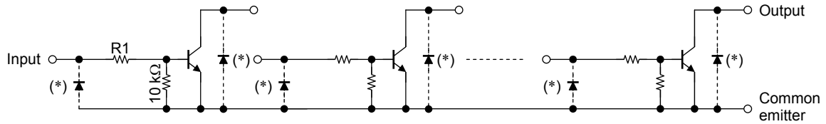
TD62503FNG
