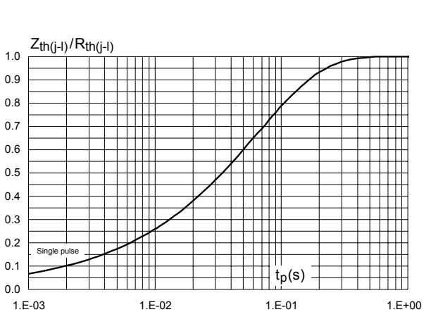
Figure 6. Relative variation of thermal impedance junction to lead versus pulse duration (SMB Flat, SMB Flat Notch)
