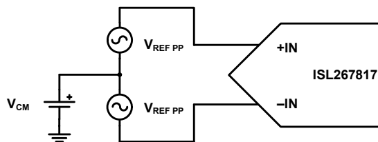
FIGURE 27. DIFFERENTIAL INPUT SIGNALING
