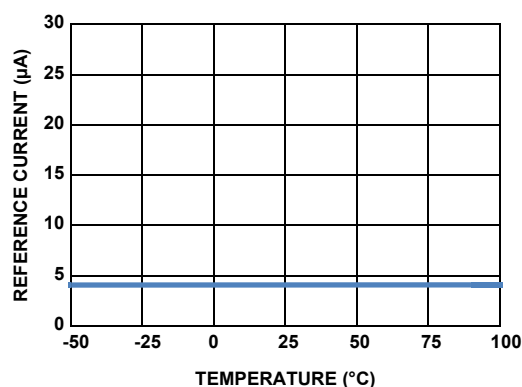
FIGURE 24. REFERENCE CURRENT vs TEMPERATURE (CODE = FF8h)
