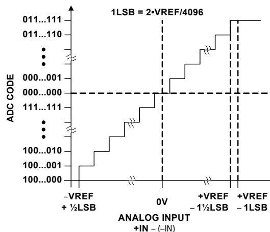
FIGURE 26. IDEAL TRANSFER CHARACTERISTICS
