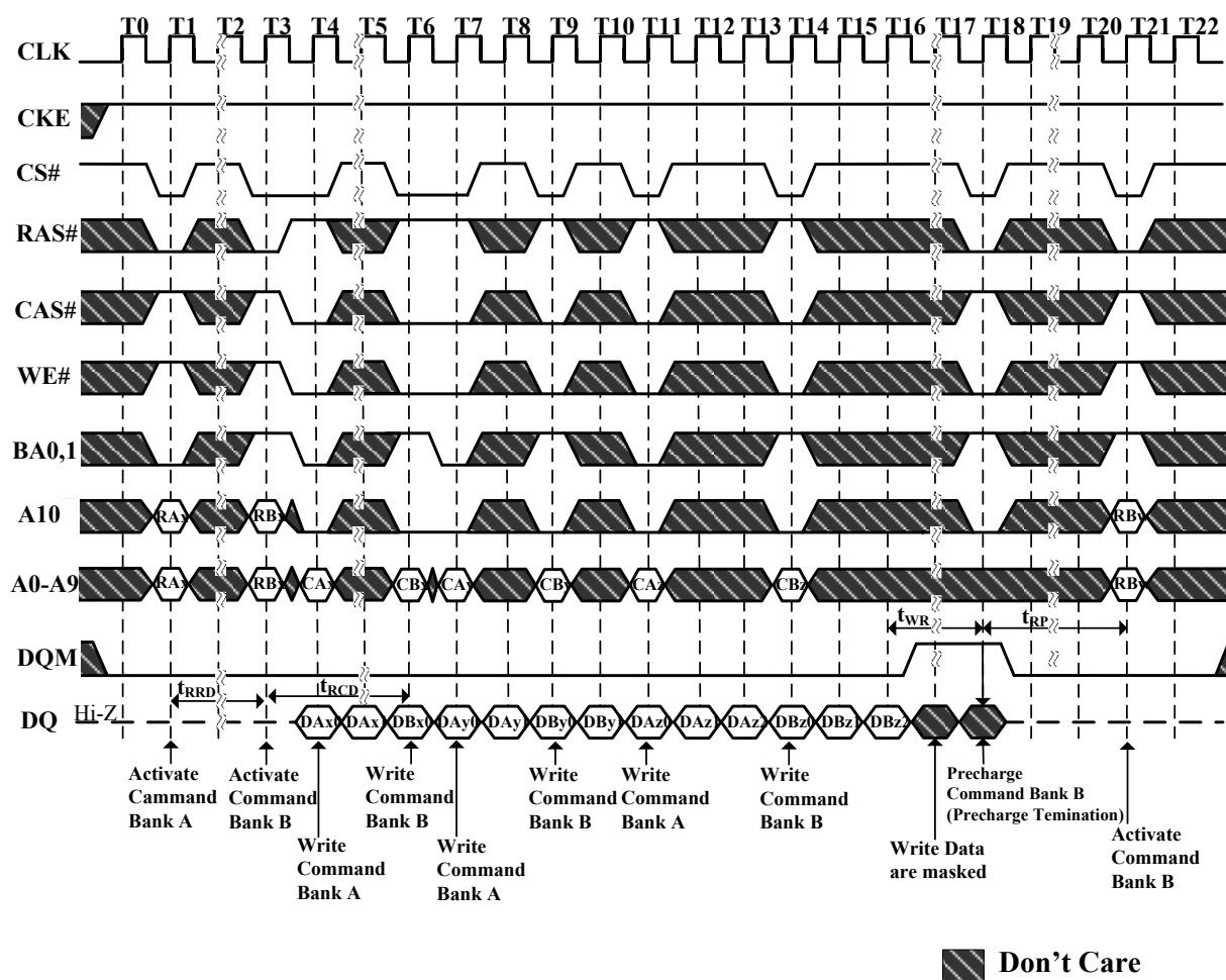
Figure 41. Full Page Random Column Write (Burst Length=Full Page)
