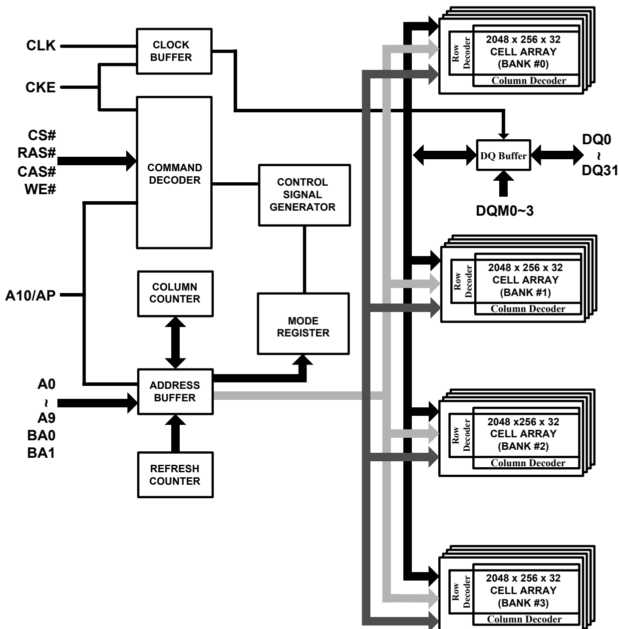
Figure 2. Block Diagram
