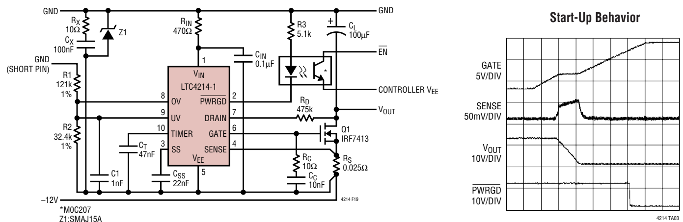
Figure 19. -12V/2A Hot Swap Controller
