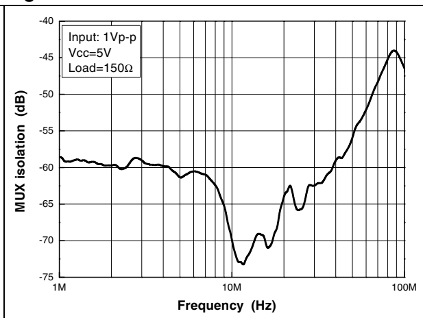
Figure 12. MUX isolation
