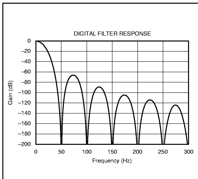
FIGURE 4. Digital Filter Response ( 50\text{Hz} ).
