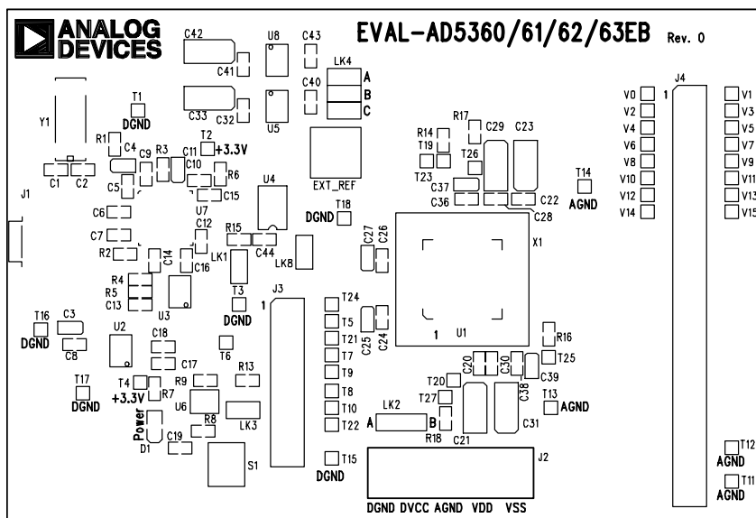
EVAL-AD5360/61/62/63EB Rev. 0 (Component Side View)
