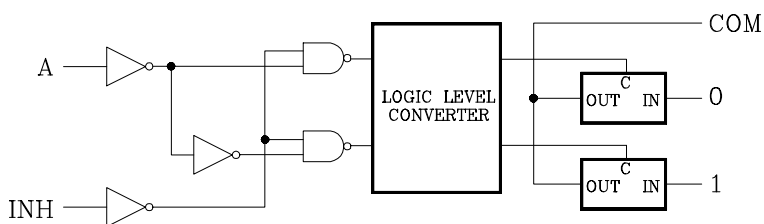
LOGIC DIAGRAM
