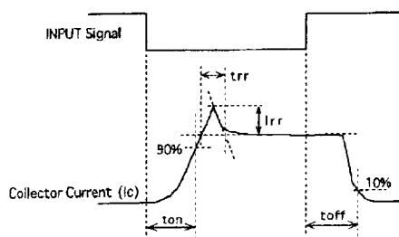
Fig.4 Definition of switching time
