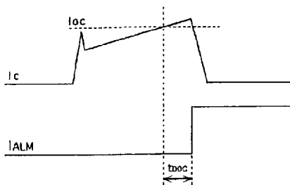
Fig.2 Definition of OC delay time
