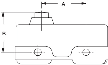
FIG. 3 Stub Plunger
