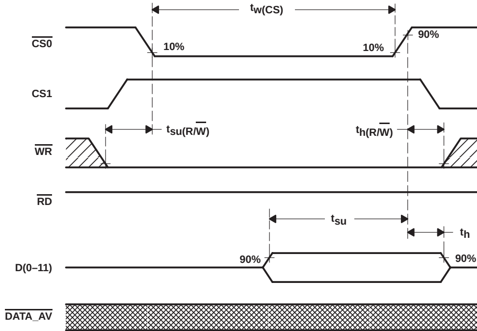
Figure 12. Write Timing Diagram Using \overline{R/W} ( \overline{CS0} -controlled)
