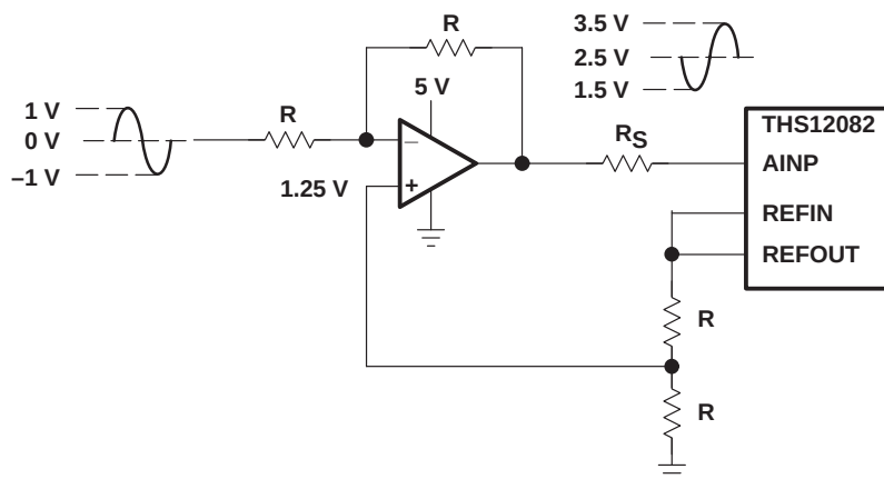
Figure 17. Level-Shift for DC-Coupled Input
