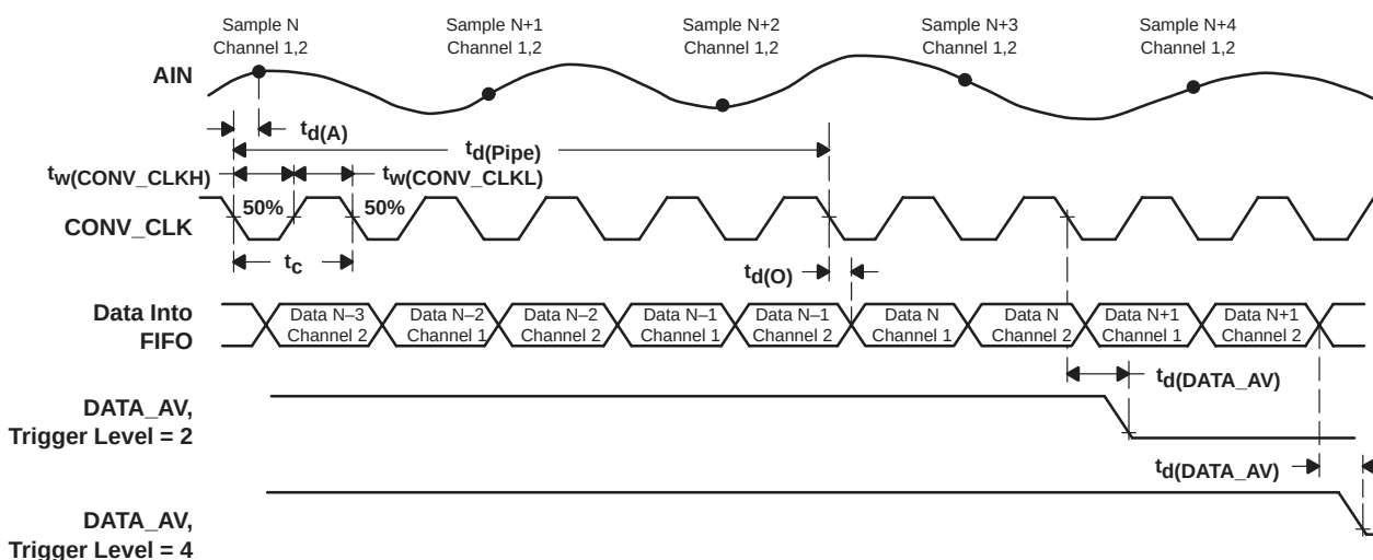
Figure 3. Timing of Continuous Conversion Mode (2-channel operation)
