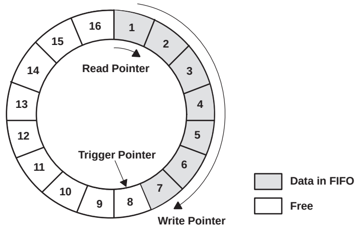
Figure 4. Circular Buffer
