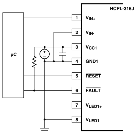
Figure 70. Local shutdown, local reset configuration.
