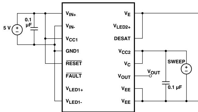
Figure 43. UVLO threshold test circuit.
