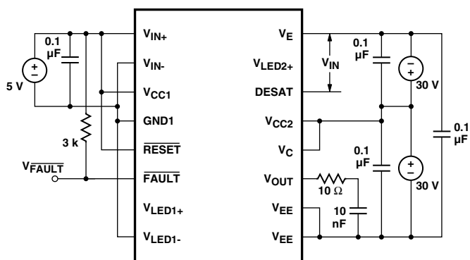
Figure 47. t_{DESAT(\overline{FAULT})} test circuit.
