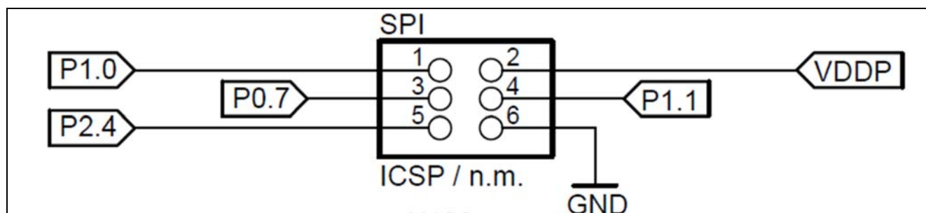
Figure 6 ICSP connector
