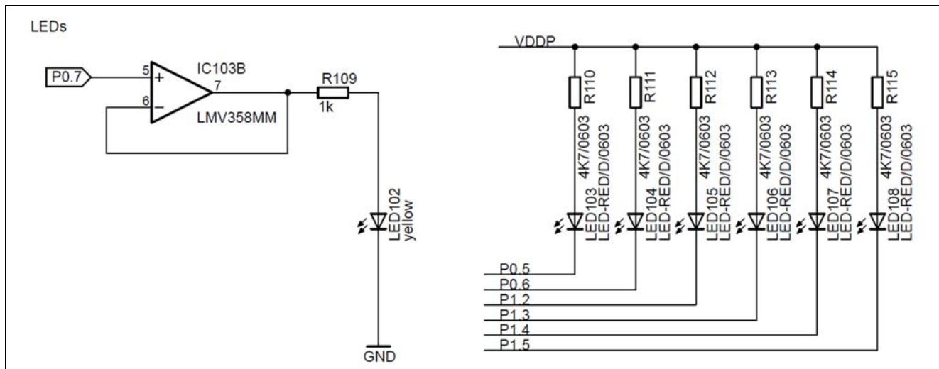
Figure 7 LEDs Circuit
