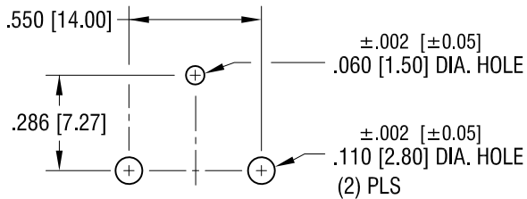
MOUNTING LAYOUT
