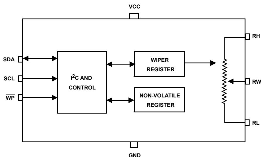
FIGURE 1. BLOCK DIAGRAM
