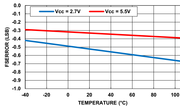
FIGURE 7. FSERROR vs TEMPERATURE FOR 50kΩ
