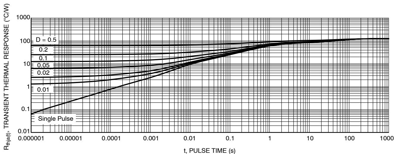
Figure 15. Thermal Response
