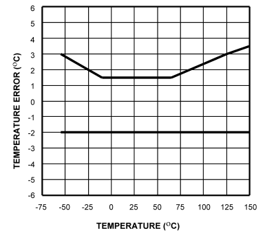
Temperature Error
