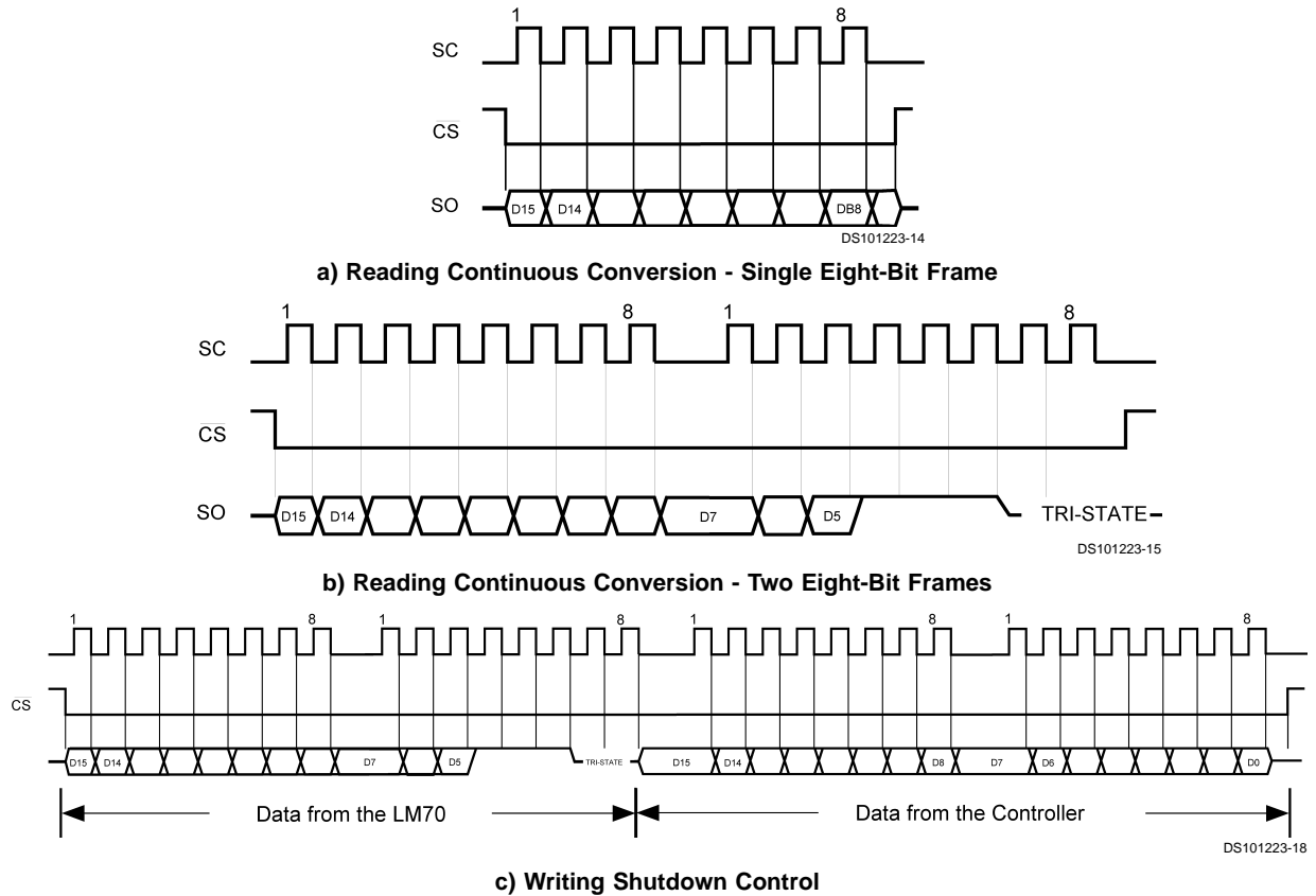
FIGURE 7. Timing Diagrams
