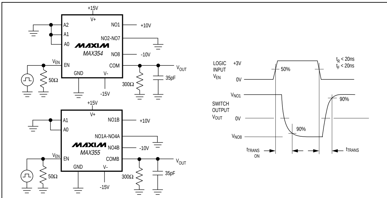
Figure 1. Transition Time
