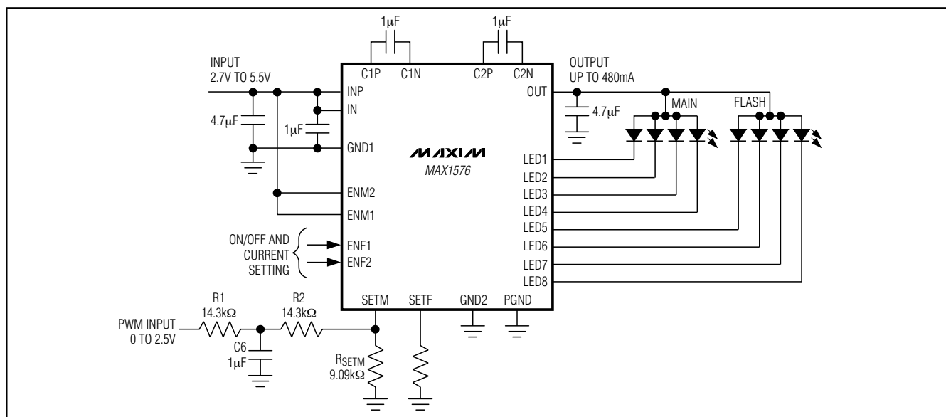
Figure 5. Dimming Using Filtered PWM Signal
