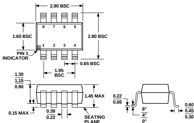
Figure 48. 8-Lead Small Outline Transistor Package [SOT-23] (RT-8) Dimensions shown in millimeters
