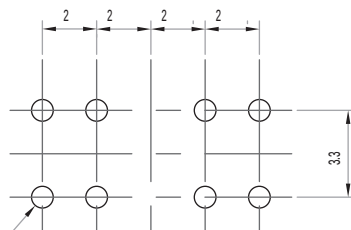
PIERCING PLAN
