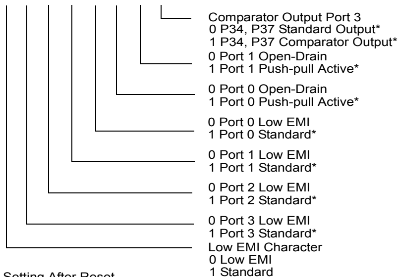
Figure 30. Port Configuration Register (PCON) (Write Only)
