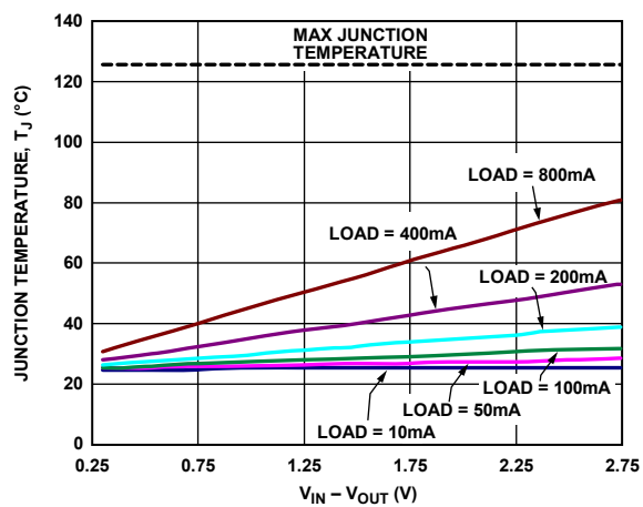
Figure 19. 1000 mm² of PCB Copper, T_B = 25^\circ\text{C} , LFCSP
