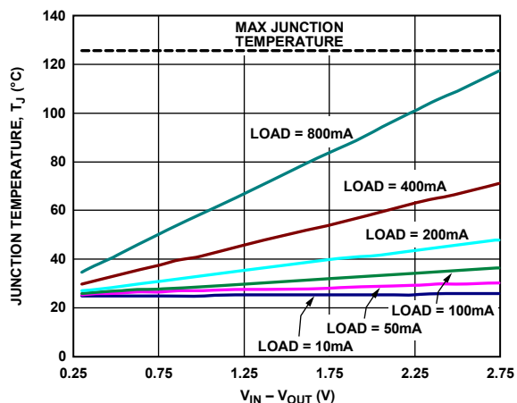
Figure 11. 6400 mm 2 of PCB Copper, T_A = 25^\circ\text{C} , LFCSP
