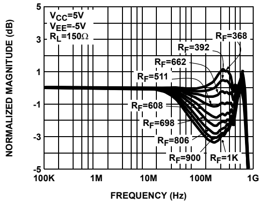
FIGURE 1. FREQUENCY RESPONSE AS THE FUNCTION OF R_F
