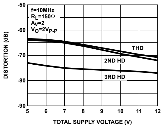
FIGURE 19. DISTORTION vs POWER SUPPLY VOLTAGE
