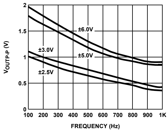
FIGURE 15. V_{OUT-P} vs FREQUENCY AND V_{CC} , V_{EE}
