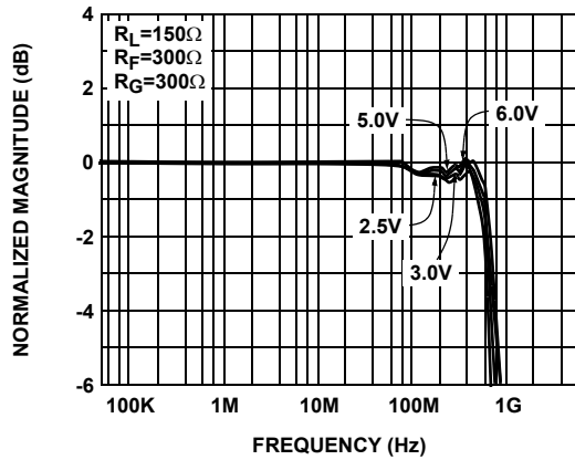
FIGURE 7. FREQUENCY RESPONSE AS THE FUNCTION OF THE POWER SUPPLY VOLTAGE
