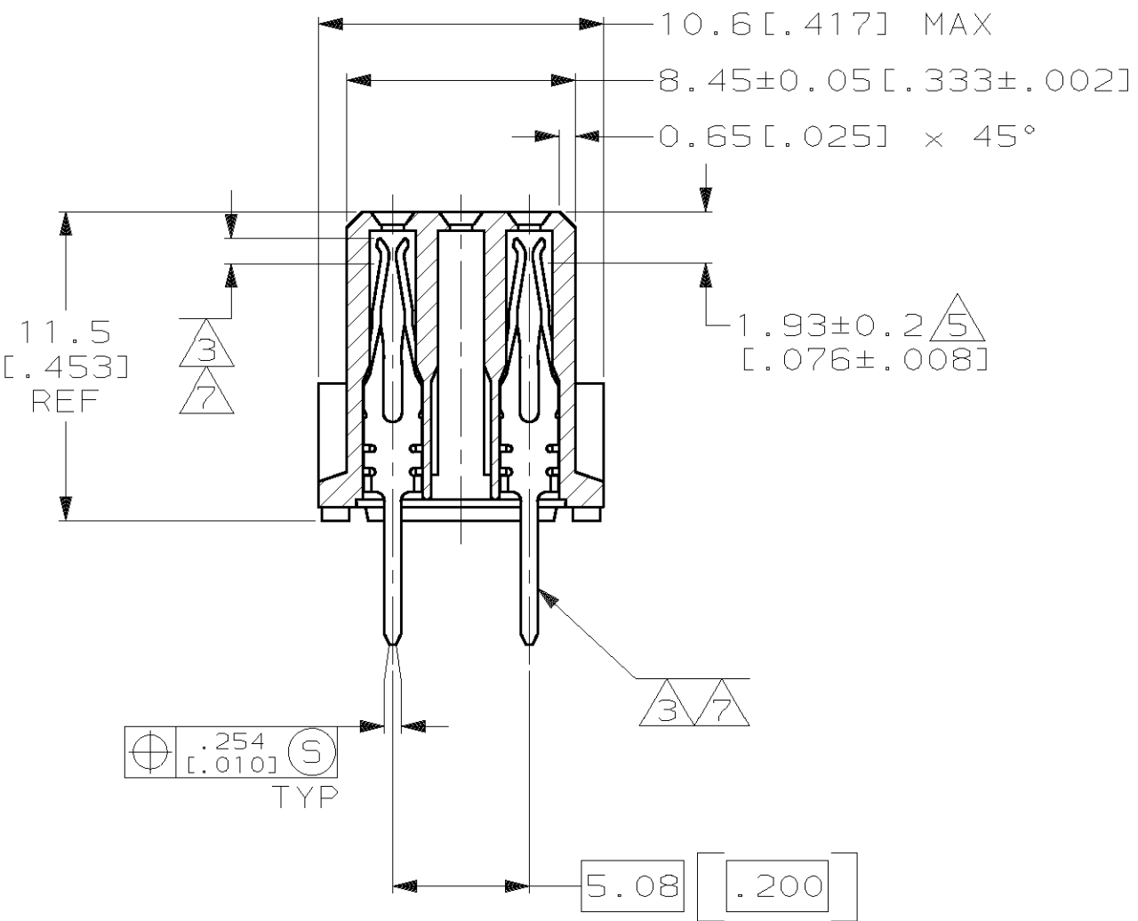
SECTION X-X
