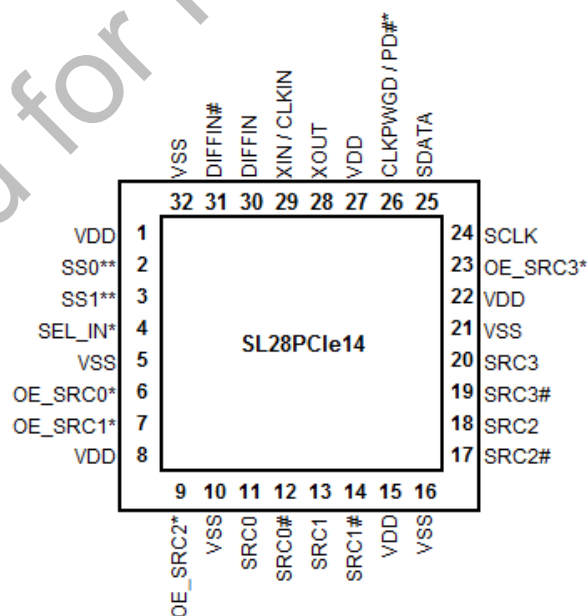
Pin Configuration
