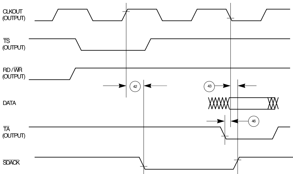
Figure 39. \overline{SDACK} Timing Diagram—Peripheral Write, \overline{TA} Sampled Low at the Falling Edge of the Clock
