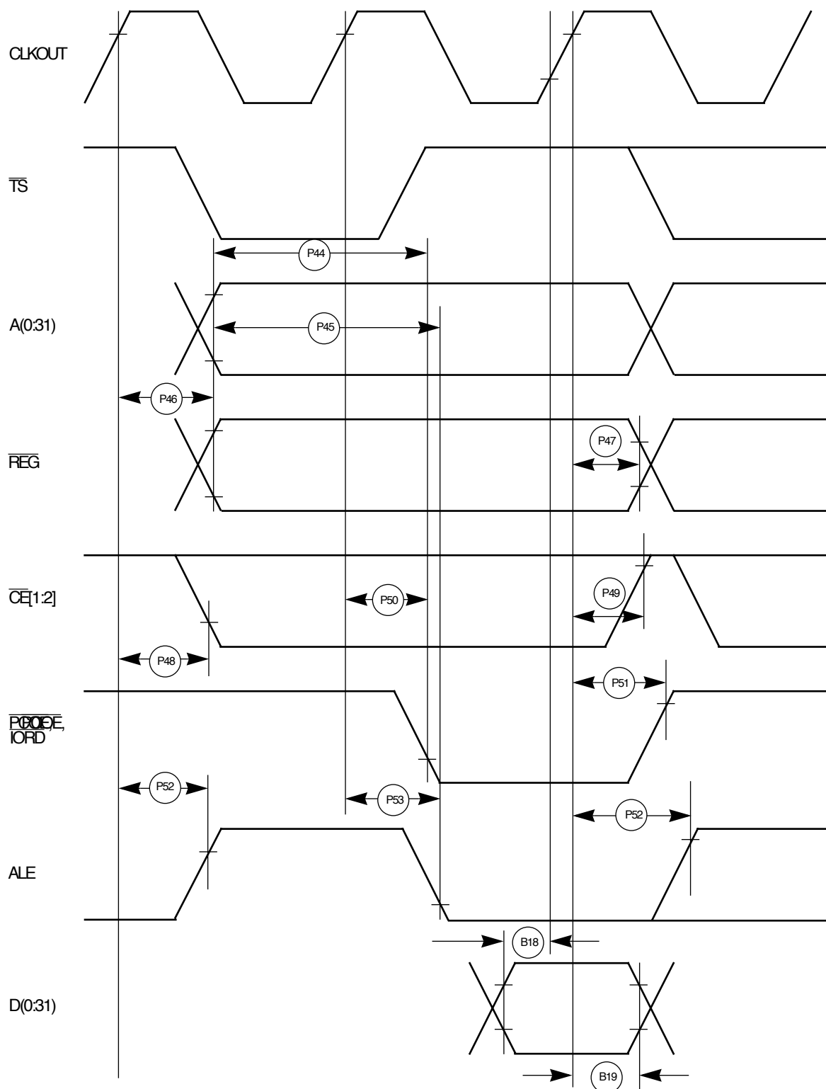
Figure 22. PCMCIA Access Cycles Timing Diagram (External Bus Read)
