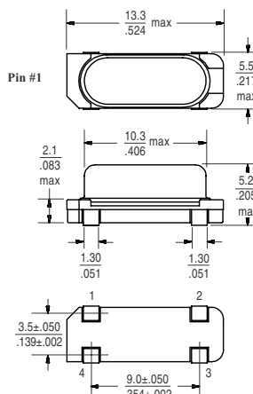
49SNC package
