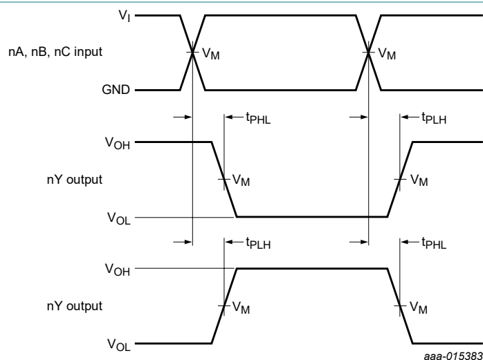
Fig. 11. Input nA, nB and nC to output nY propagation delay times
