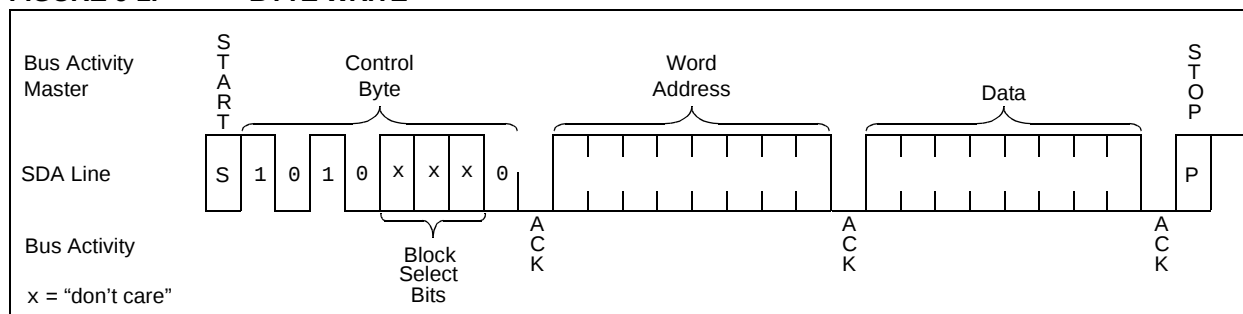
FIGURE 6-1: BYTE WRITE
