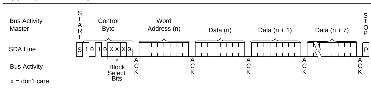
FIGURE 6-2: PAGE WRITE
