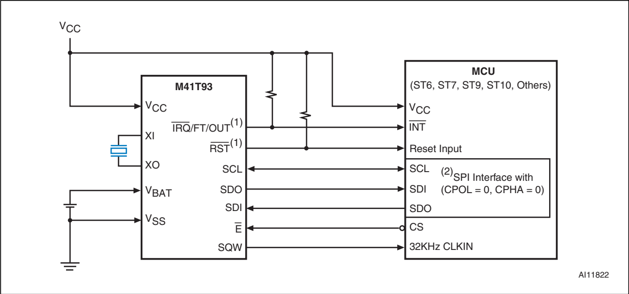
Figure 5. Hardware hookup
