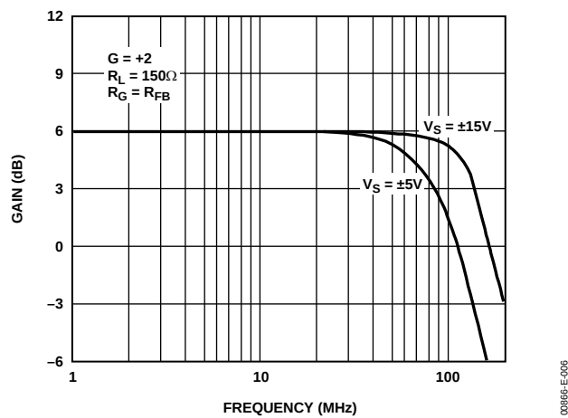
Figure 6. Frequency Response
