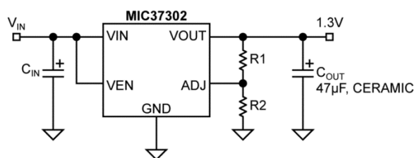
Adjustable Regulator
