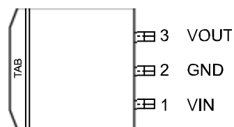
S-PAK-3 (R)
