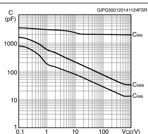
Figure 13. Capacitance variation
