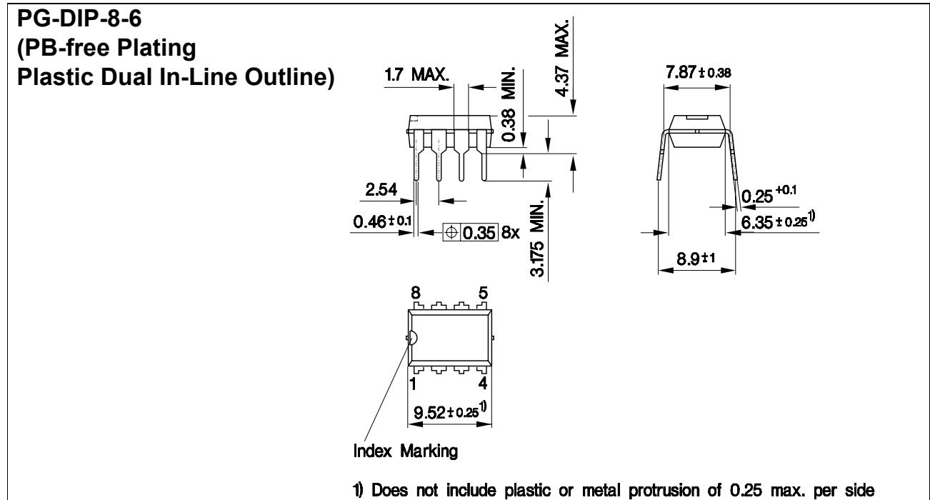
Figure 23 PG-DIP-8-6 (PB-free Plating Plastic Dual In-Line Outline)
