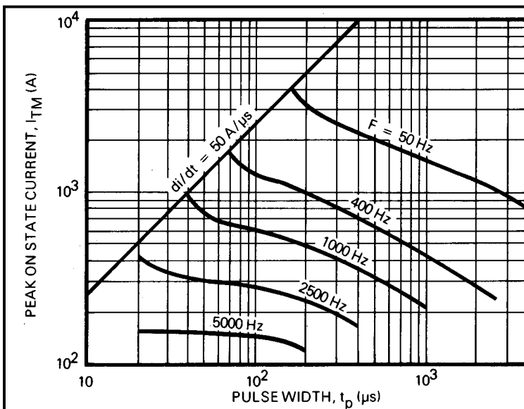
Fig.14 Maximum allowable peak on-state current vs pulse width for T_{case} = 65^\circ\text{C}
