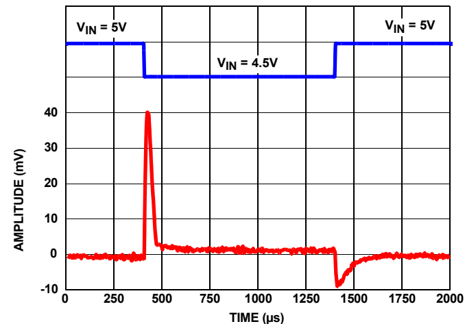
FIGURE 127. LINE TRANSIENT RESPONSE WITH 10\mu F LOAD
