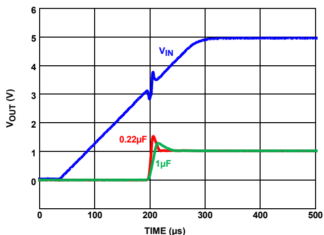
FIGURE 12. TURN-ON TIME
