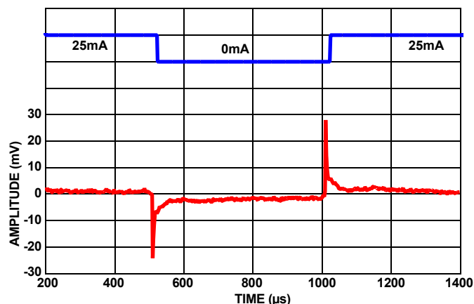
FIGURE 95. LOAD TRANSIENT RESPONSE AT 25mA LOAD AT 1\mu F
