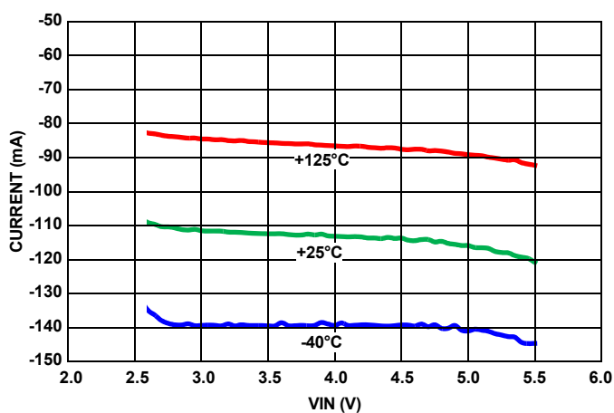
FIGURE 86. SHORT-CIRCUIT TO GND
