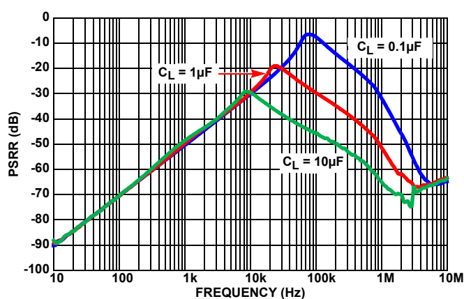
FIGURE 31. RIPPLE REJECTION AT DIFFERENT CAPACITIVE LOADS
