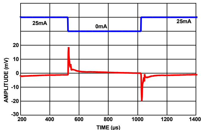
FIGURE 112. LOAD TRANSIENT RESPONSE AT 25mA LOAD AT 1 \mu F
