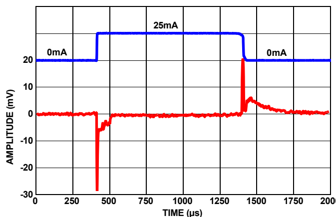
FIGURE 78. LOAD TRANSIENT RESPONSE AT 25mA LOAD AT 1 \mu F
