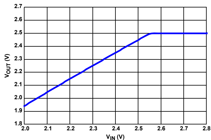
FIGURE 83. DROPOUT (10mA SOURCED LOAD)
