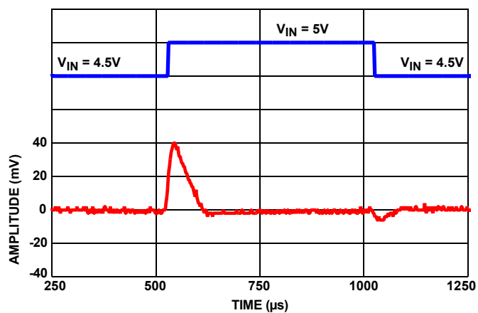
FIGURE 93. LINE TRANSIENT RESPONSE WITH 10\mu F LOAD
