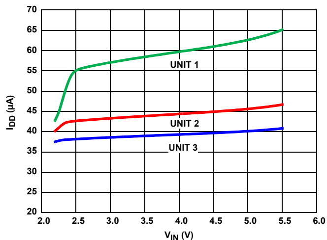
FIGURE 3. I_{IN} vs V_{IN} , THREE UNITS
