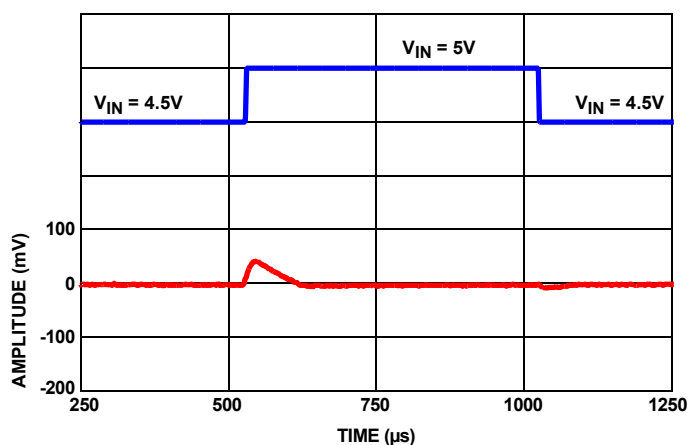
FIGURE 110. LINE TRANSIENT RESPONSE WITH 10\mu F LOAD
