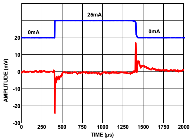
FIGURE 44. LOAD TRANSIENT RESPONSE AT 25mA LOAD AT 1μF
