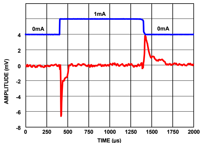
FIGURE 79. LOAD TRANSIENT RESPONSE AT 1mA LOAD AT 1 \mu F
