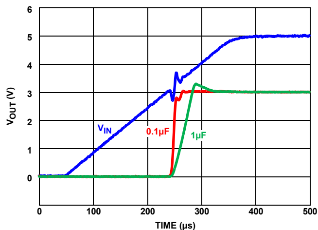
FIGURE 97. TURN-ON TIME
