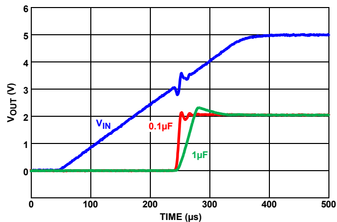
FIGURE 63. TURN-ON TIME
