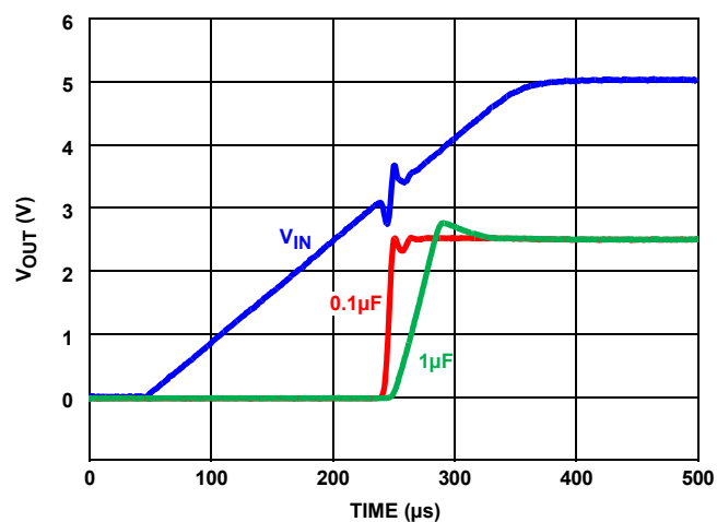
FIGURE 80. TURN-ON TIME
