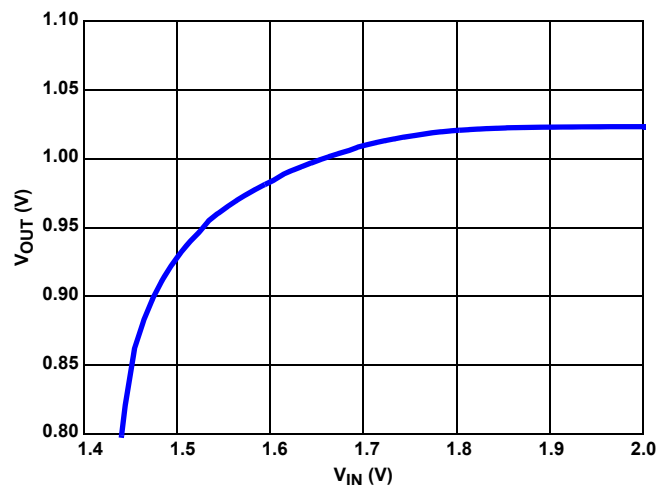
FIGURE 15. DROPOUT (10mA SOURCED LOAD)
