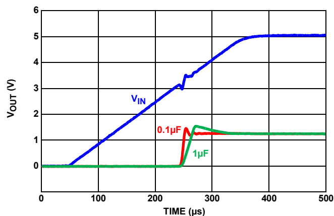
FIGURE 29. TURN-ON TIME
