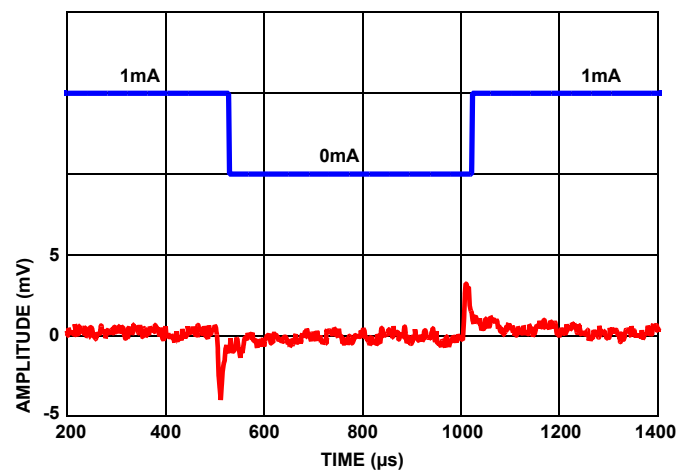
FIGURE 96. LOAD TRANSIENT RESPONSE AT 1mA LOAD AT 1\mu F
