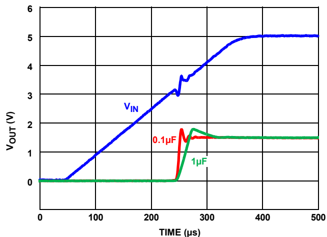
FIGURE 46. TURN-ON TIME
