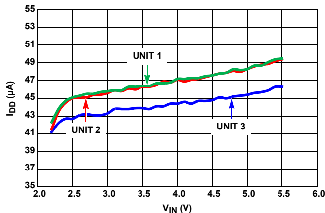
FIGURE 20. I_{IN} vs V_{IN} , THREE UNITS
