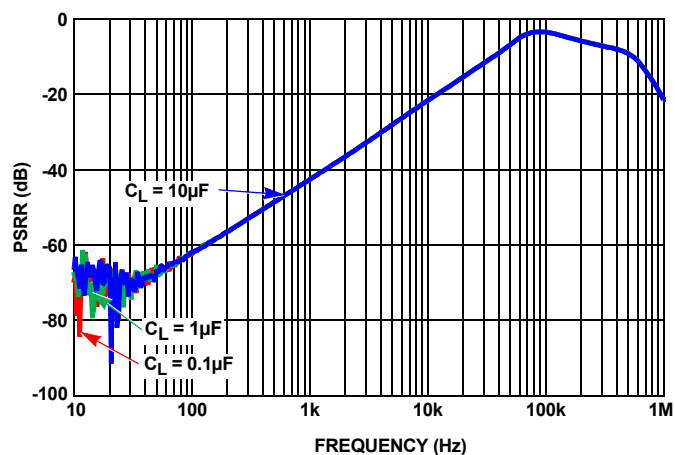
FIGURE 99. RIPPLE REJECTION AT DIFFERENT CAPACITIVE LOADS
