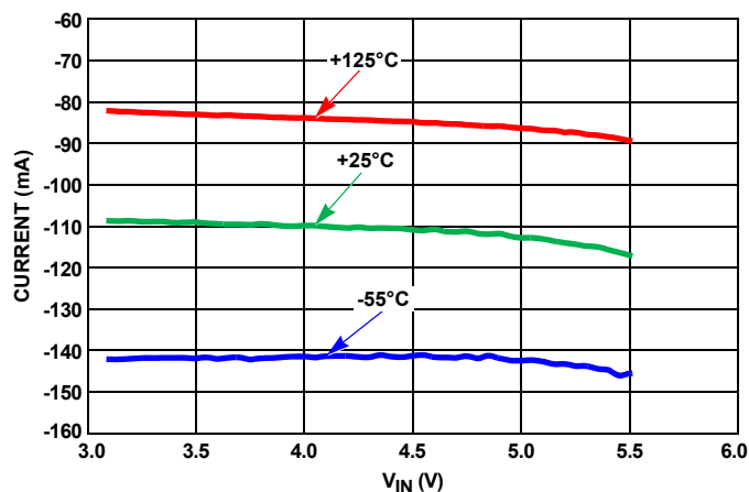
FIGURE 103. SHORT-CIRCUIT TO GND
