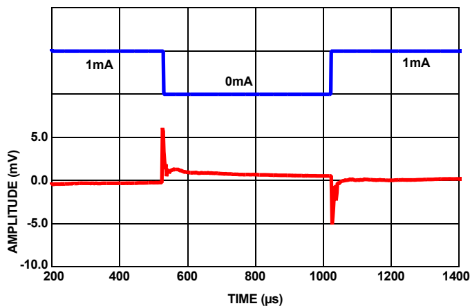
FIGURE 113. LOAD TRANSIENT RESPONSE AT 1mA LOAD AT 1 \mu F
