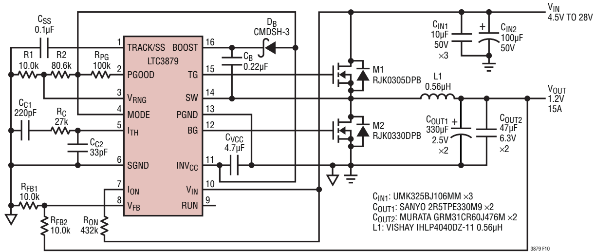
Figure 10. Design Example: 1.2V/15A at 400kHz
