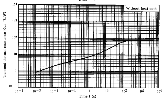
R_{th(t)} - t
