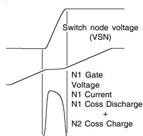
Figure 6 – Q_{OSS} Waveforms
