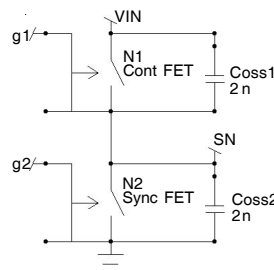
Figure 5 – Q_{OSS} Equivalent Circuit
