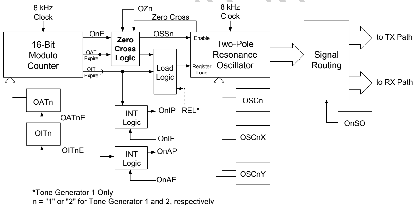
Figure 11. Simplified Tone Generator Diagram
