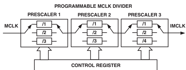
Figure 10. MCLK Divider
