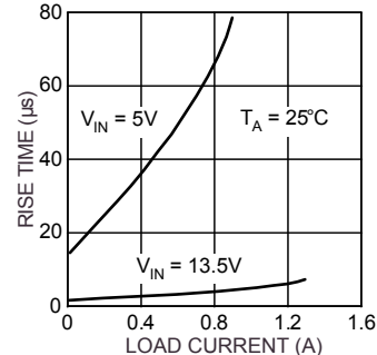
Rise Time vs. Load Current
