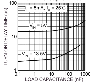
Turn-On Delay Time vs. Load Capacitance
