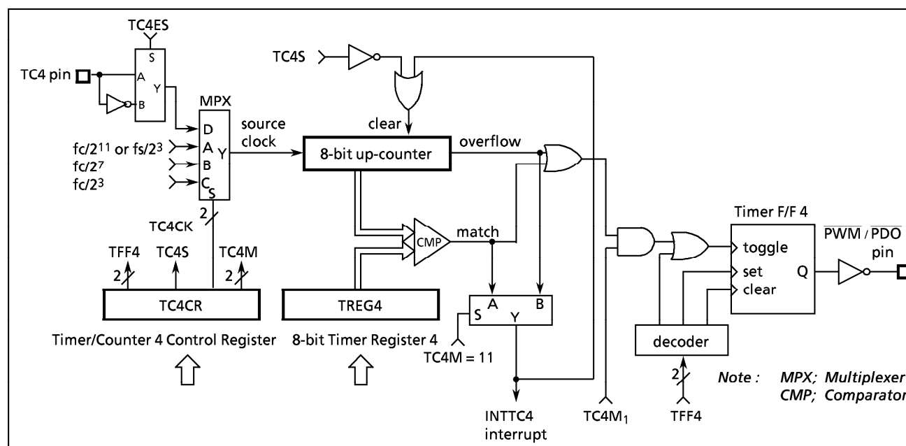
Figure 2-32. Timer/Counter 4
