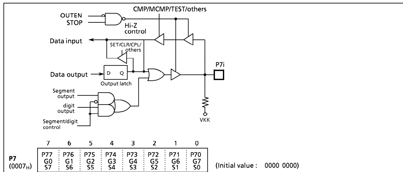
Figure 2-10. Port P7
