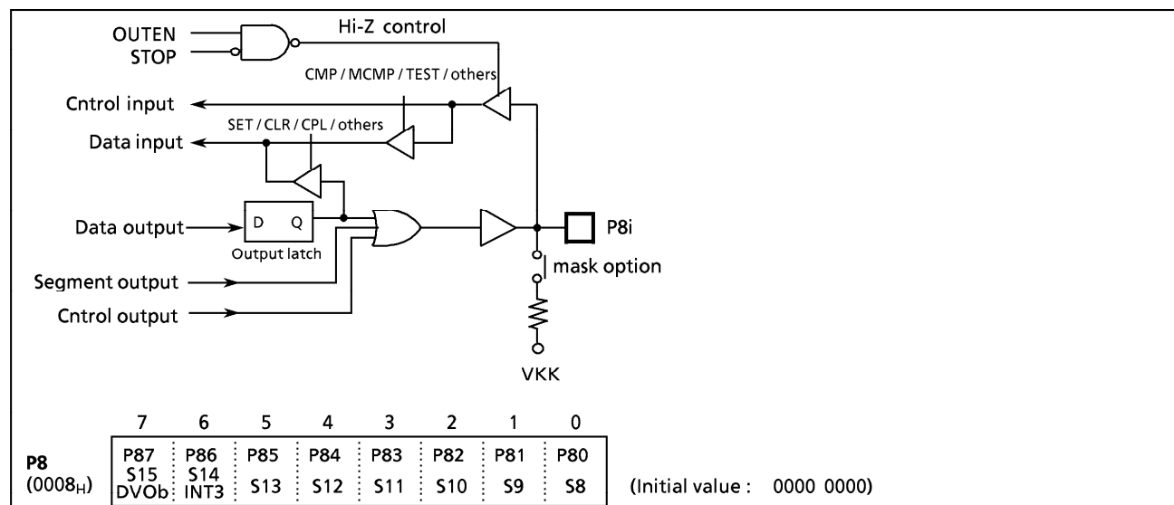
Figure 2-11. Port P8
