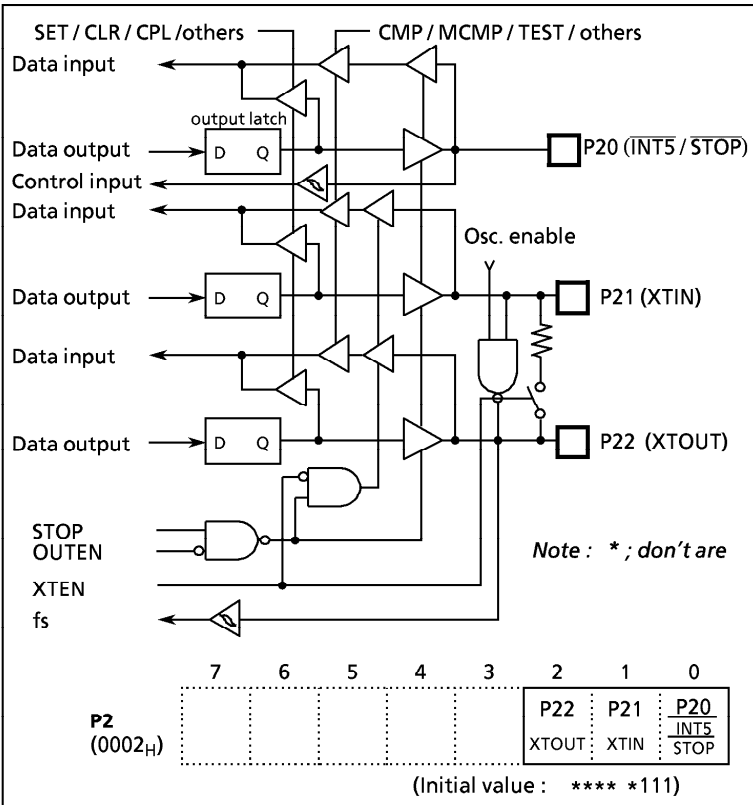
Figure 2-5. Port P2
