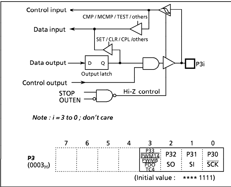
Figure 2-6. Port P3
