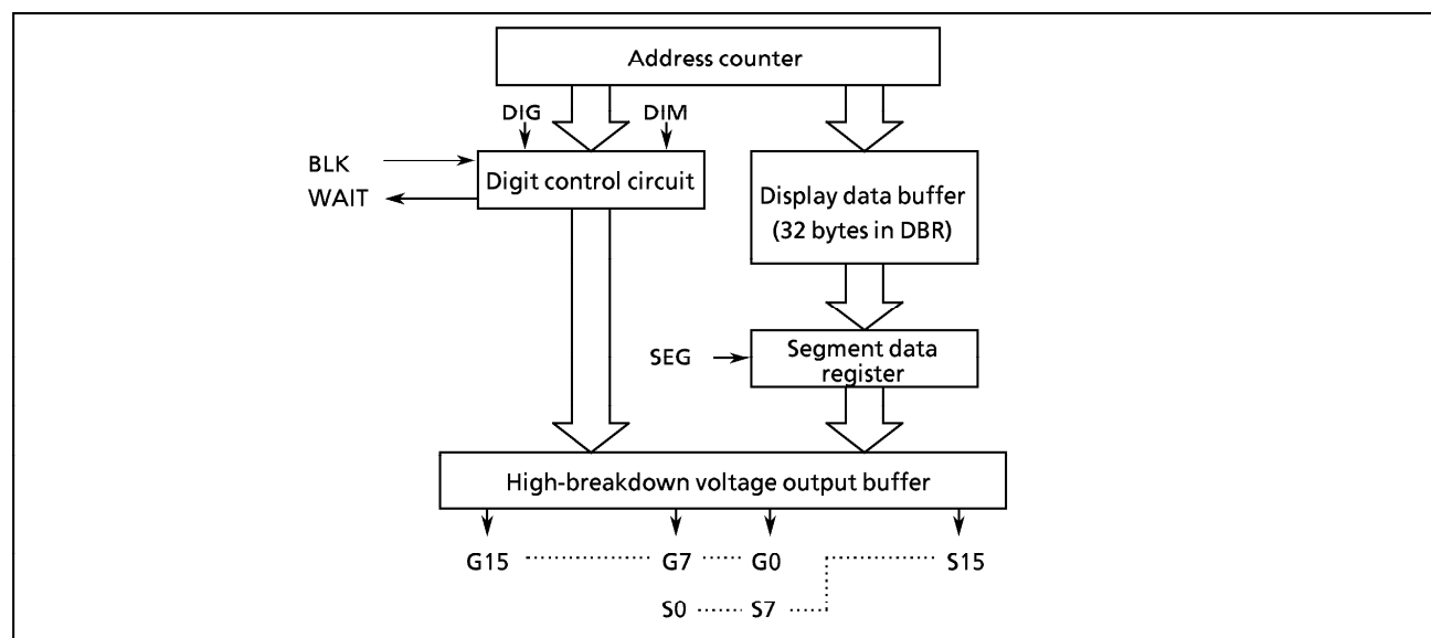
Figure 2-53. VFT
