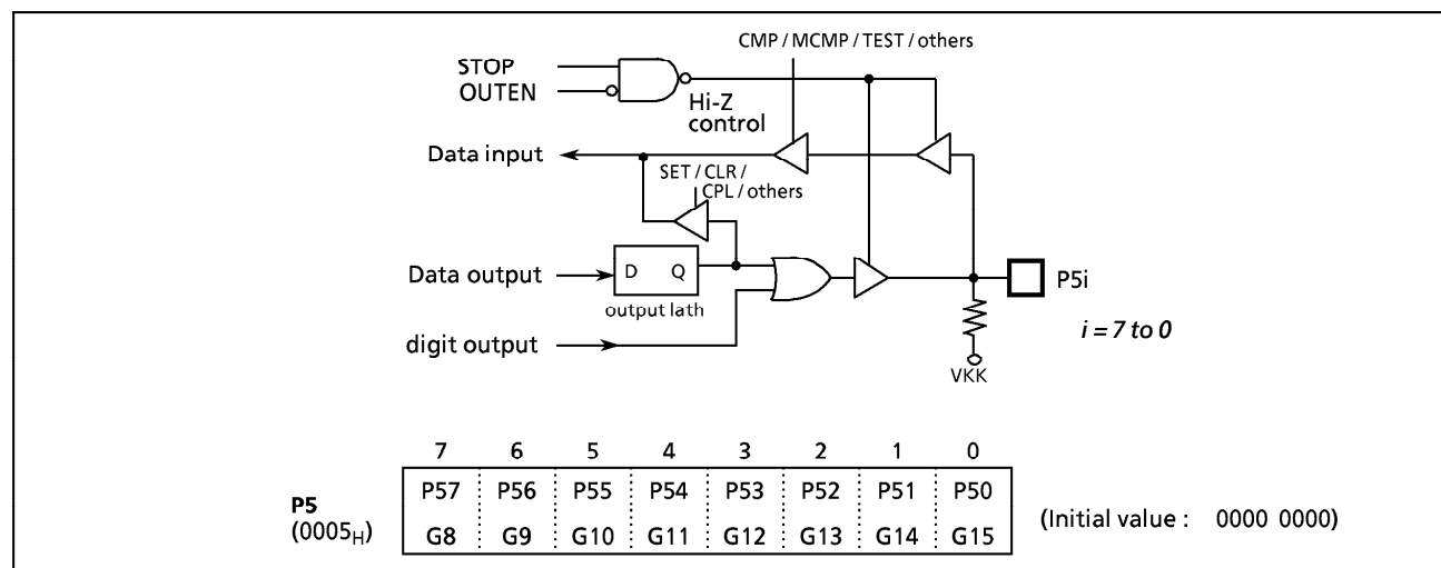
Figure 2-8. P5 Port
