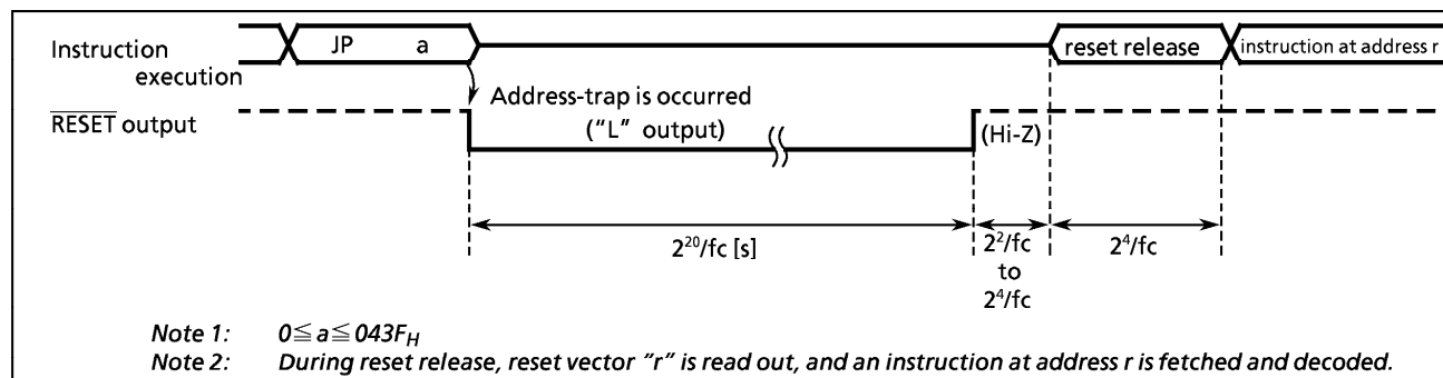
Figure 1-31. Address-Trap-Reset
