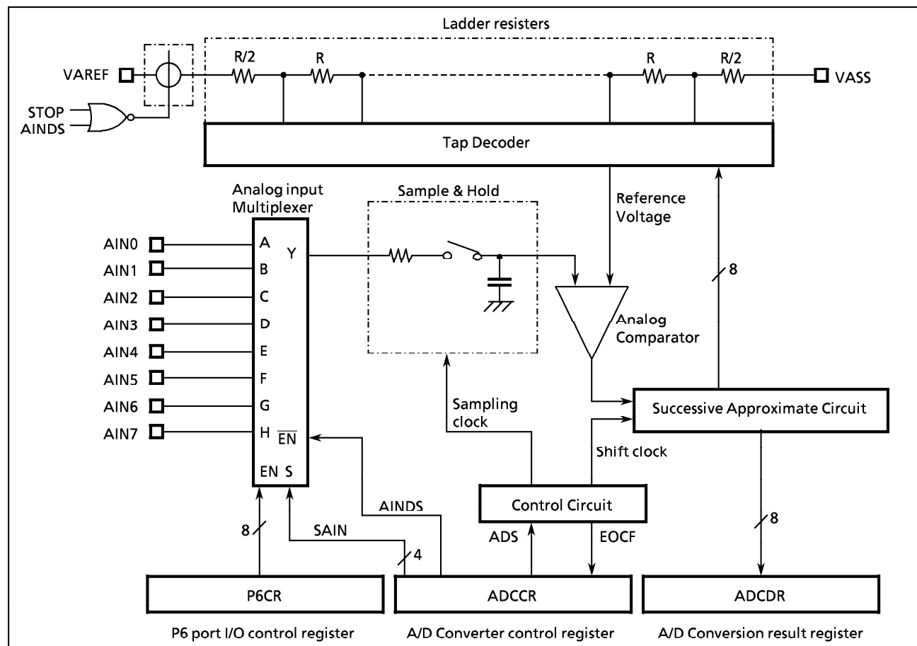
Figure 2-46. A/D Converter
