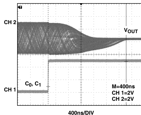
FIGURE 42. DISABLE RESPONSE
