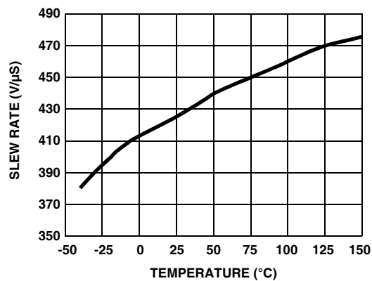
FIGURE 44. SLEW RATE vs TEMPERATURE
