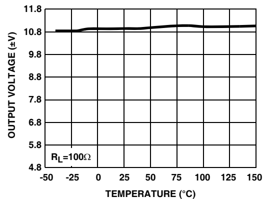
FIGURE 46. OUTPUT VOLTAGE vs TEMPERATURE
