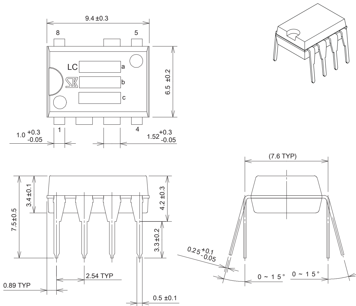
Package Diagram DIP8 package
