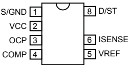
Pin-out Diagram
