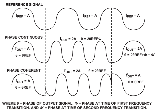
Figure 31. Difference Between a Phase Continuous Frequency Change and a Phase Coherent Frequency Change
