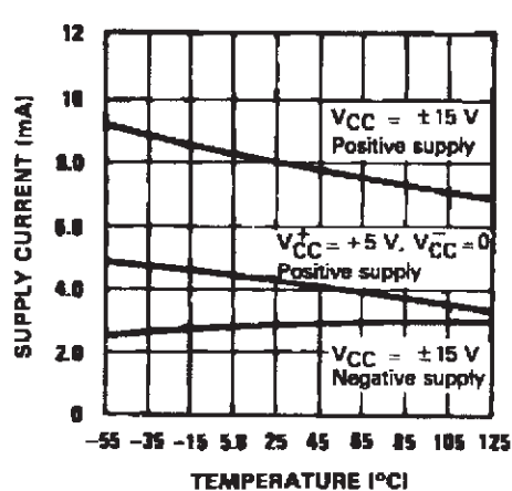
SUPPLY CURRENT
