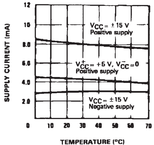
SUPPLY CURRENT
